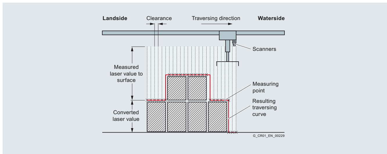
Measurement of the height of the container stack with the laser scanner
