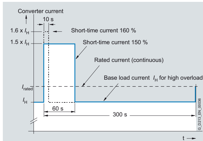
High overload
