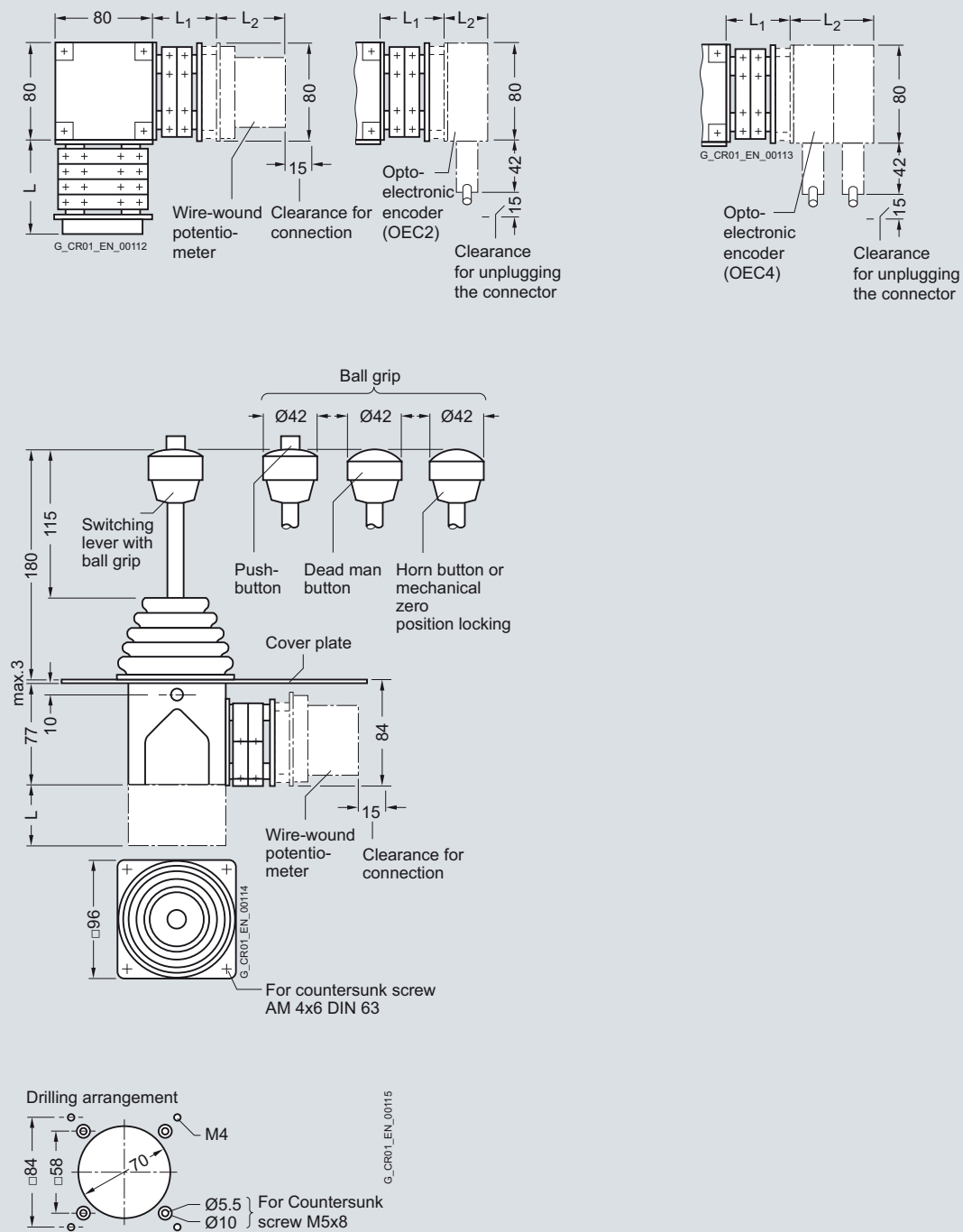
Double master controller 3SJ3
