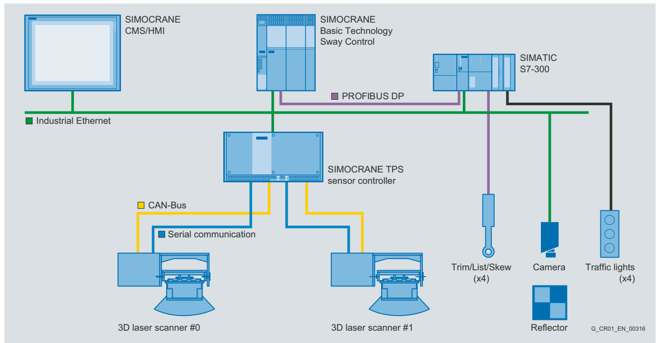
Topology of semi-automated STS crane
