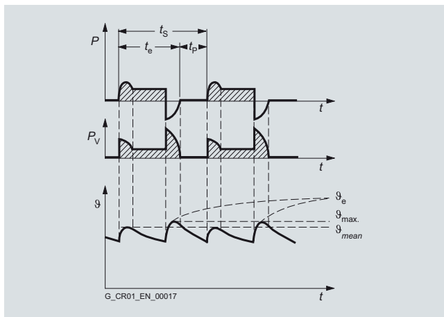
Intermittent duty S5
