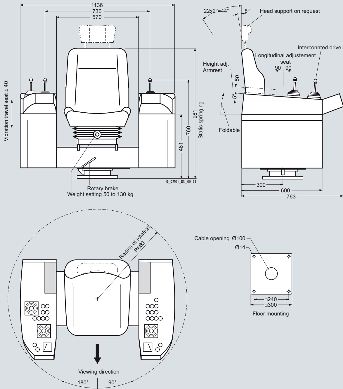
Dimension drawing crane controller 3SJ9
