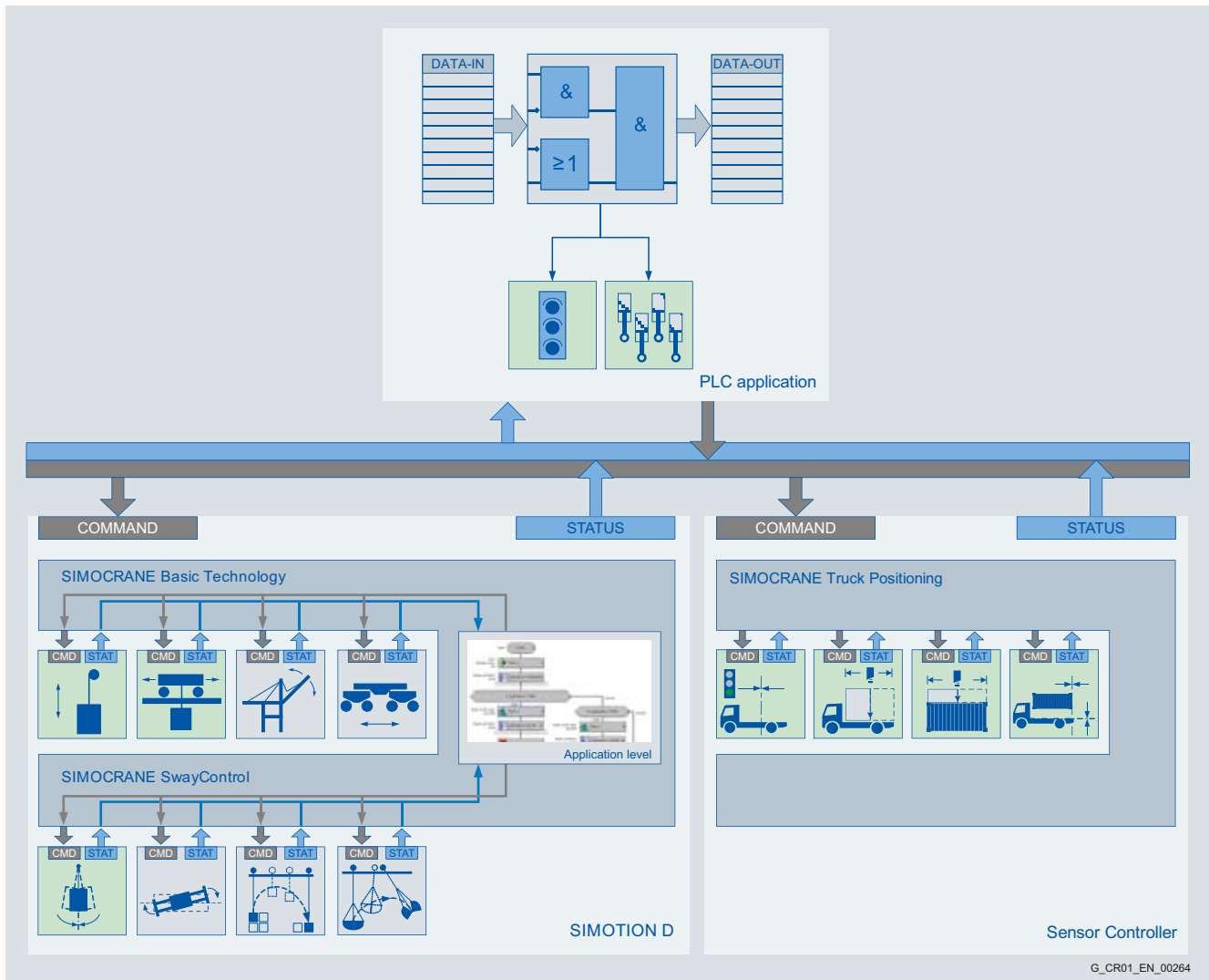
Function blocks of the application example for a semi-automated STS crane
