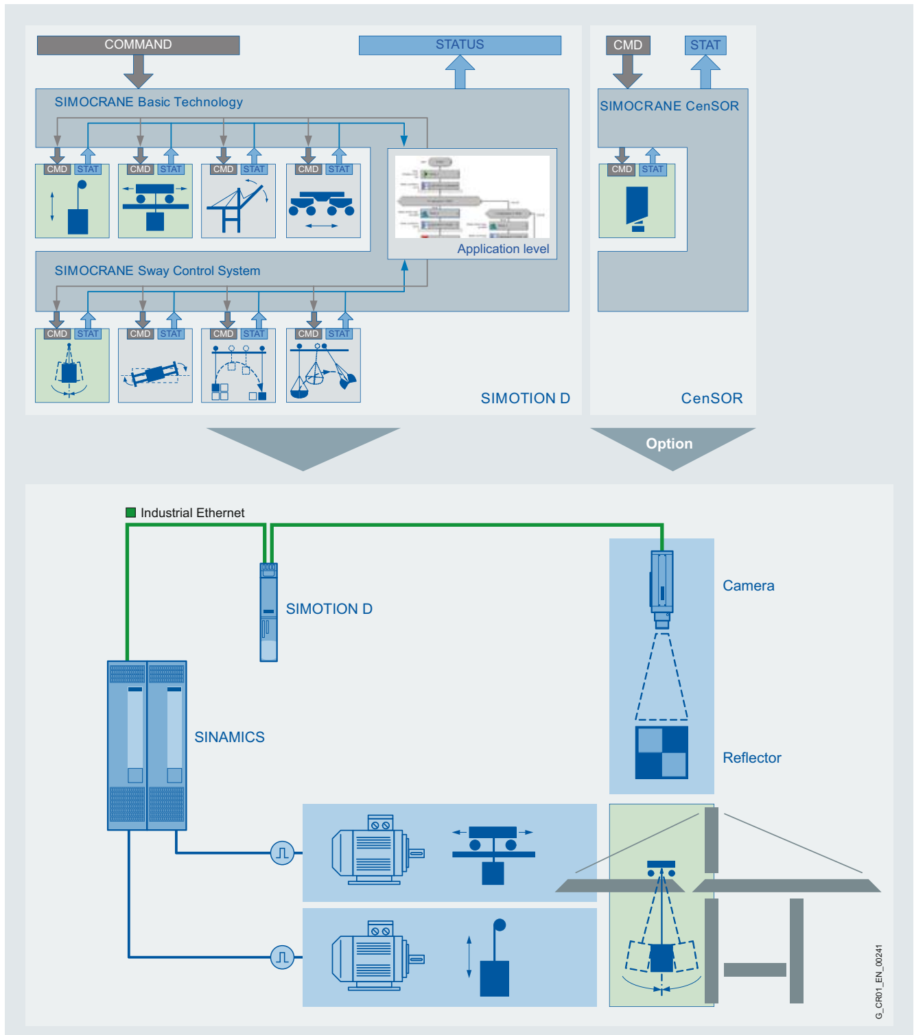
Configuration of SIMOCRANE SC integrated for an STS application
