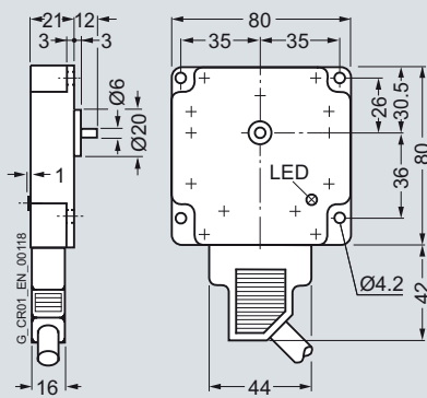
Opto-electronic encoder 6GA4 603-2AA00, -3AA00, -4AA00
