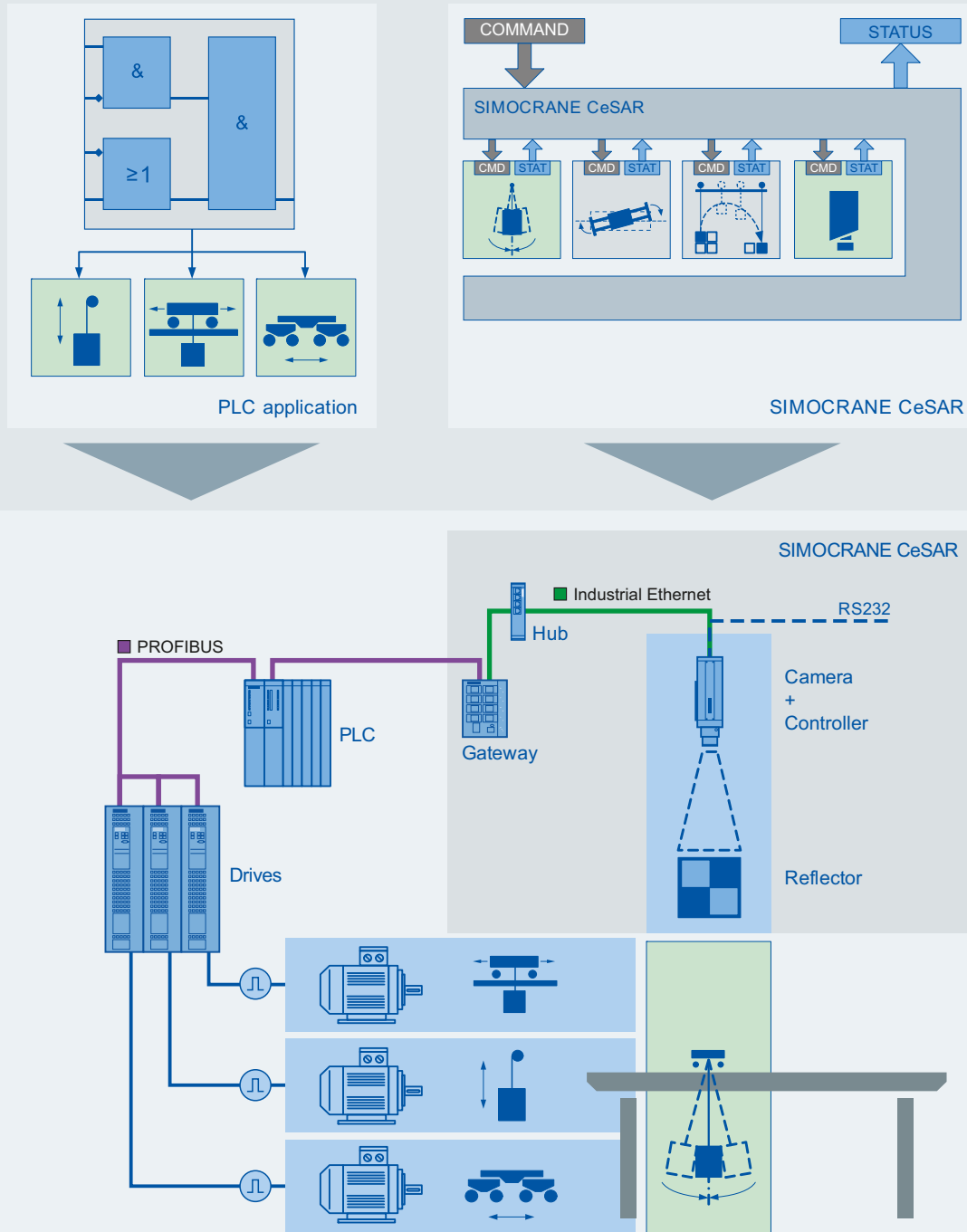
Configuration of SIMOCRANE CeSAR standalone for an overhead bridge crane application
