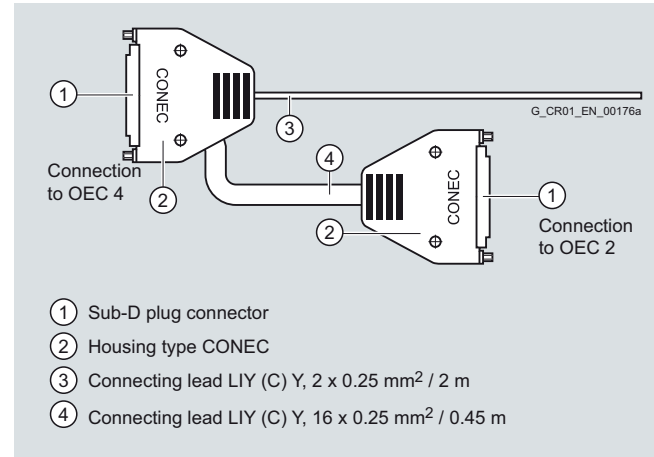
Cable for connecting OEC 4 to OEC 2: 3SX4 237
