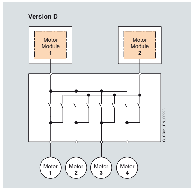
Function diagram for version D
