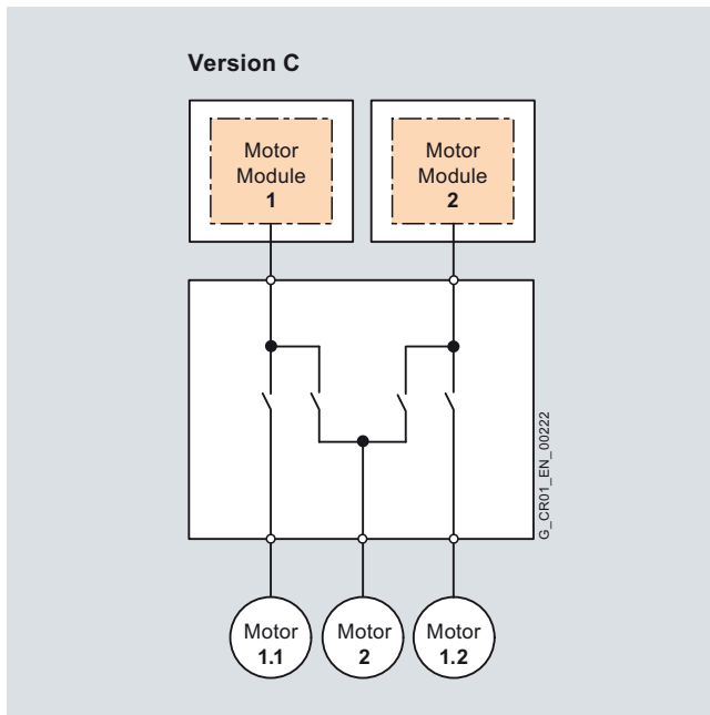
Function diagram for version C
