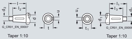
Conical shaft extension
