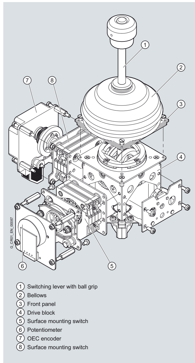
Design of double master controller 3SJ3
