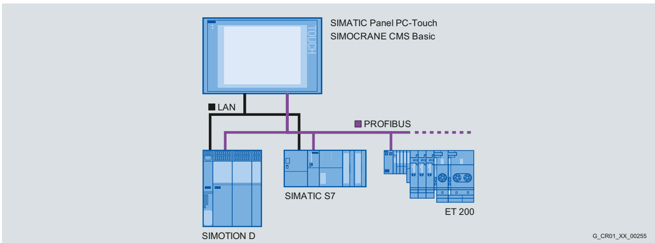
CMS single-user system (SIMOCRANE Basic)
