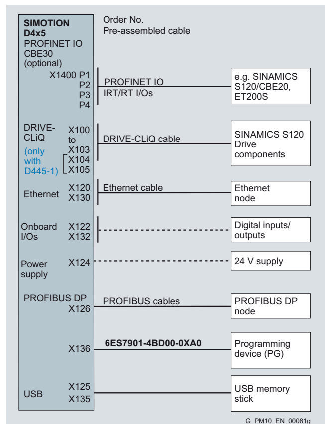
SIMOTION D4x5 connection overview
