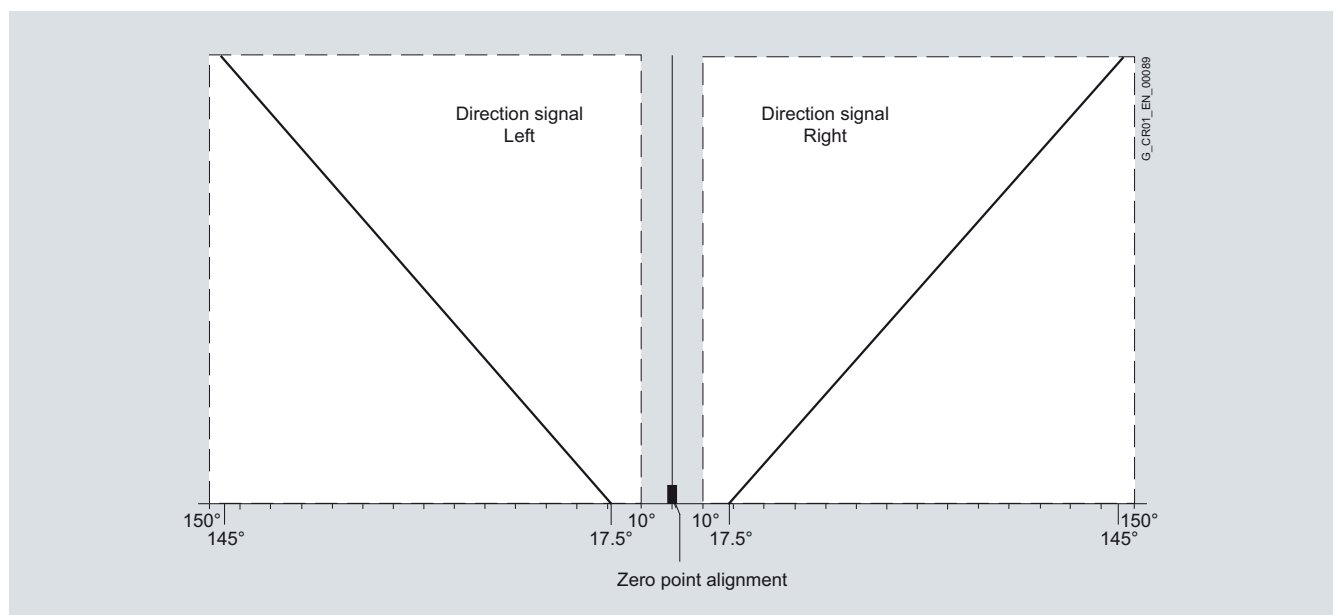
Output characteristic of the opto-electronic encoder for digital master controllers
