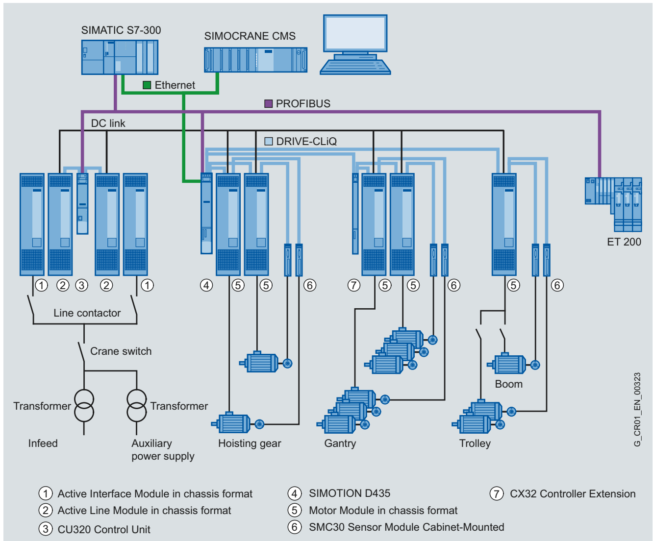
Topology of container quay crane
